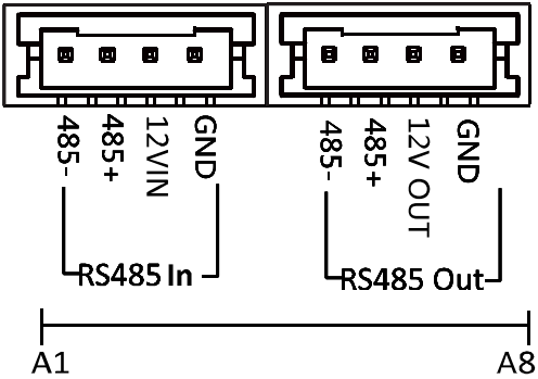
Figure 2-1 Terminals and Interfaces
