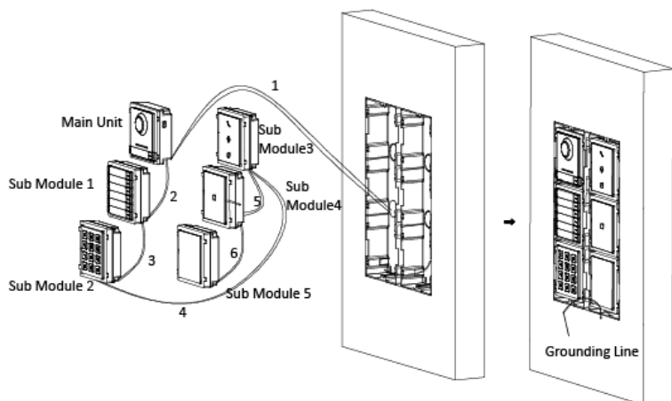
Figure 3-63 Install Mounting Frames The cables connect to each module shown as below:
